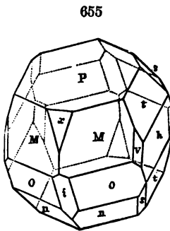
Achmatovsk.
